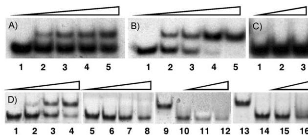
Figure 3. EMSA results showing the binding of peptides 1 , 2a – c , and 4 to dsDNA T/GAGAG . Experiments (A–C) were carried out with 45 pM ^{32}\text{P} dsDNA and analyzed by autoradiography, whereas experiments shown in (D) were carried out with 50 nM dsDNA and analyzed by SyBr-gold staining. All experiments were carried out in the following buffer solution: 18 mM Tris-HCl (pH 7.0), 50 mM KCl, 0.5 mM EDTA, 0.55 mM DTT, 1.8 mM \text{MgCl}_2 , 9% glycerol, 0.11 mg mL -1 BSA, and 4.2% NP-40. All experiments were performed in the presence 10 equivalents of \text{ZnCl}_2 except when indicated. A) Hybrid 1 in the presence of dsDNA, [ 1 ] = 0, 20, 400, 600, 1000 nM. B) Hybrid 2a in the presence of dsDNA, [ 2a ] = 0, 2, 5, 10, 15 nM. C) Control peptide 4 in the presence of dsDNA, [ 4 ] = 200, 600, 1000 nM. D) Binding of peptides: 2a , 2b , and 2c to the dsDNA; lanes 21–4: hybrid 2a , [ 2a ] = 0, 50, 100, 200 nM; lanes 5–8: hybrid 2a in the absence of \text{Zn}^{2+} , [ 2a ] = 50, 200, 300 nM; lanes 9 and 13: controls with hybrid 2a , [ 2a ] = 400 nM; lanes 10–12: hybrid 2b , [ 2b ] = 100, 300, 500 nM; lanes 14–16: hybrid 2c , [ 2c ] = 200, 500, 1000 nM. BSA = bovine serum albumin, NP-40 = Nonidet P40 (octylphenolpoly(ethyleneglycol ether)).
